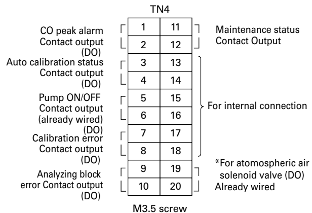
External terminal block diagram (Upper side of main unit)
