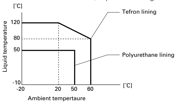
Ambient temperature-liquid temperature allowable range
