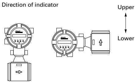
Horizontal mounting (Code 1) Vertical mounting (Code 2)
