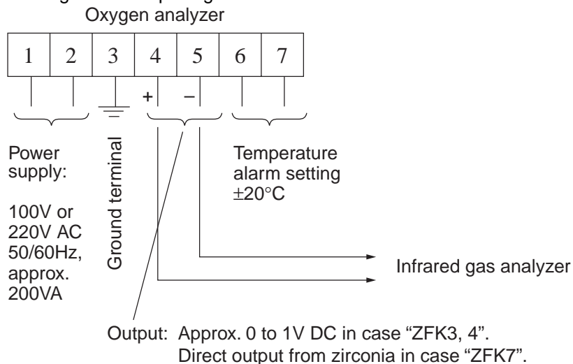
Fig. 3-1 External wiring
